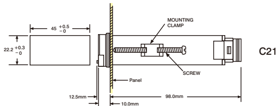
Figure 2.1 Mounting Dimensions
